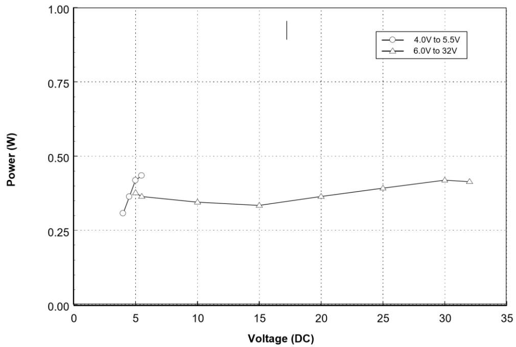
Figure 7: Average Power Consumption During Standby
