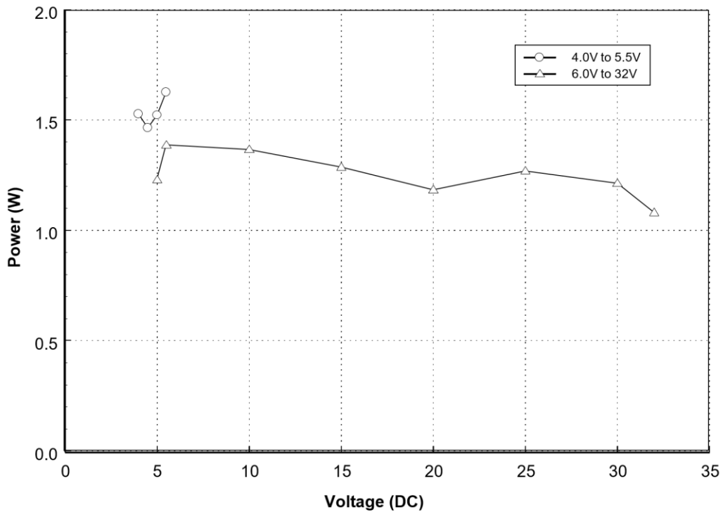
Figure 13: Average Power Consumption During an SMS Transmission
