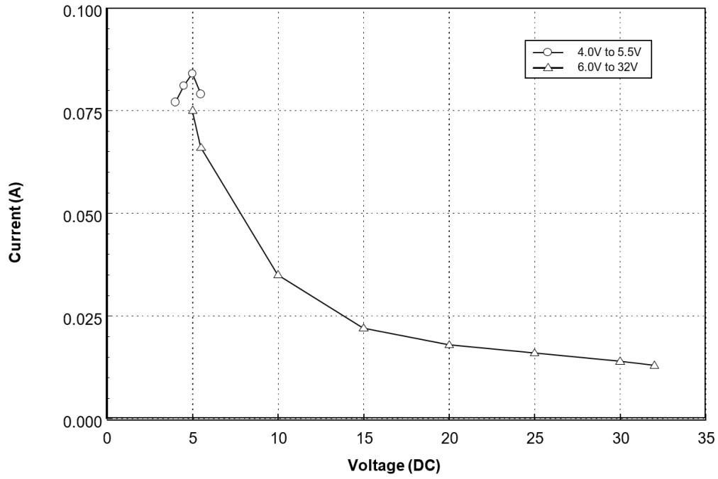
Figure 6: Average Current Drawn During Standby
