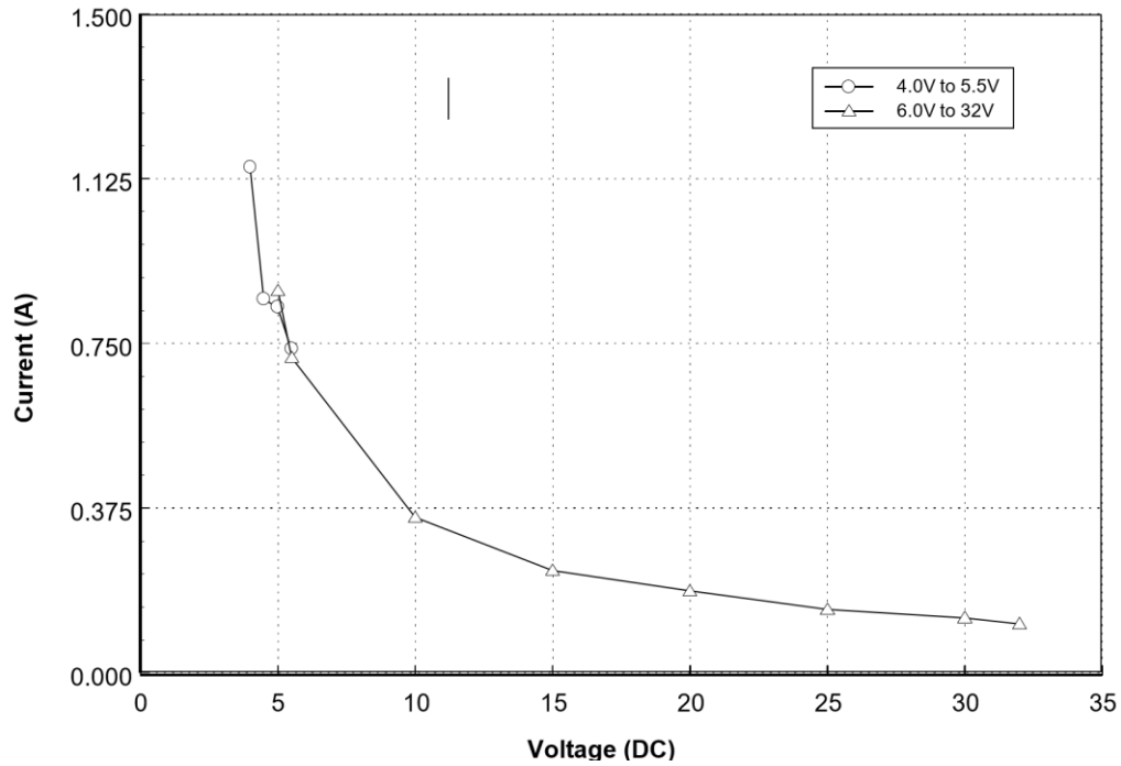
Figure 14: Average Current Drawn During a Voice Call Using DPL Handset
