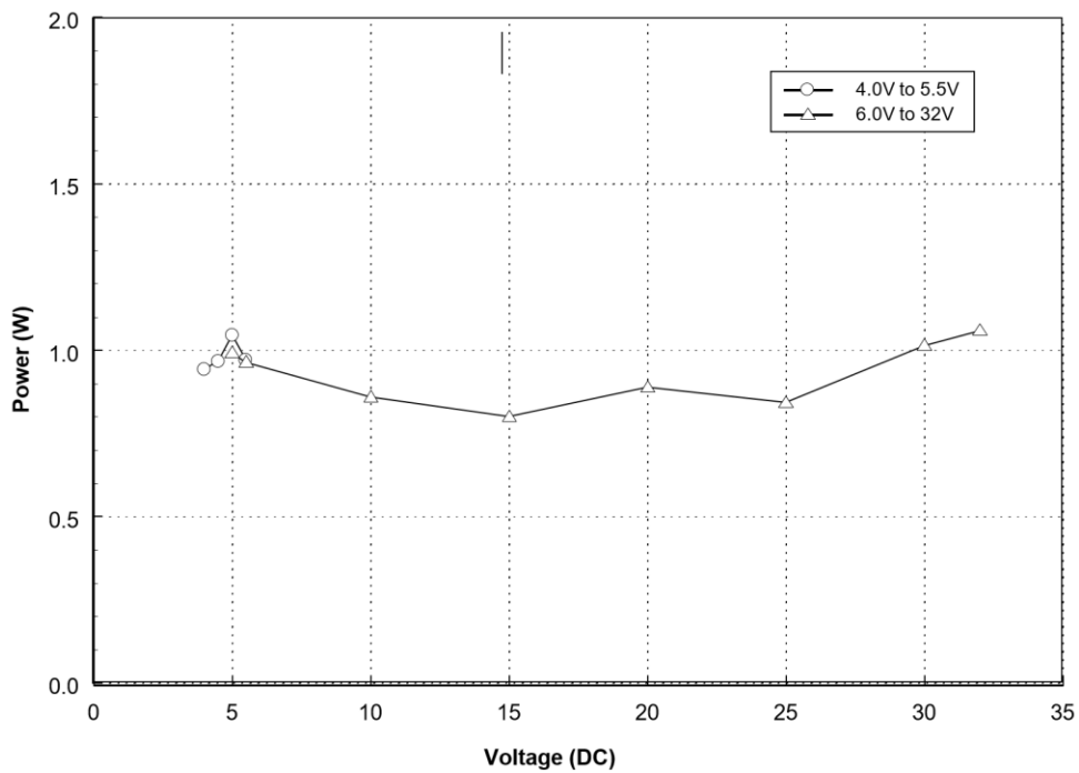
Figure 11: Average Power Consumption During an SBD Transmission
