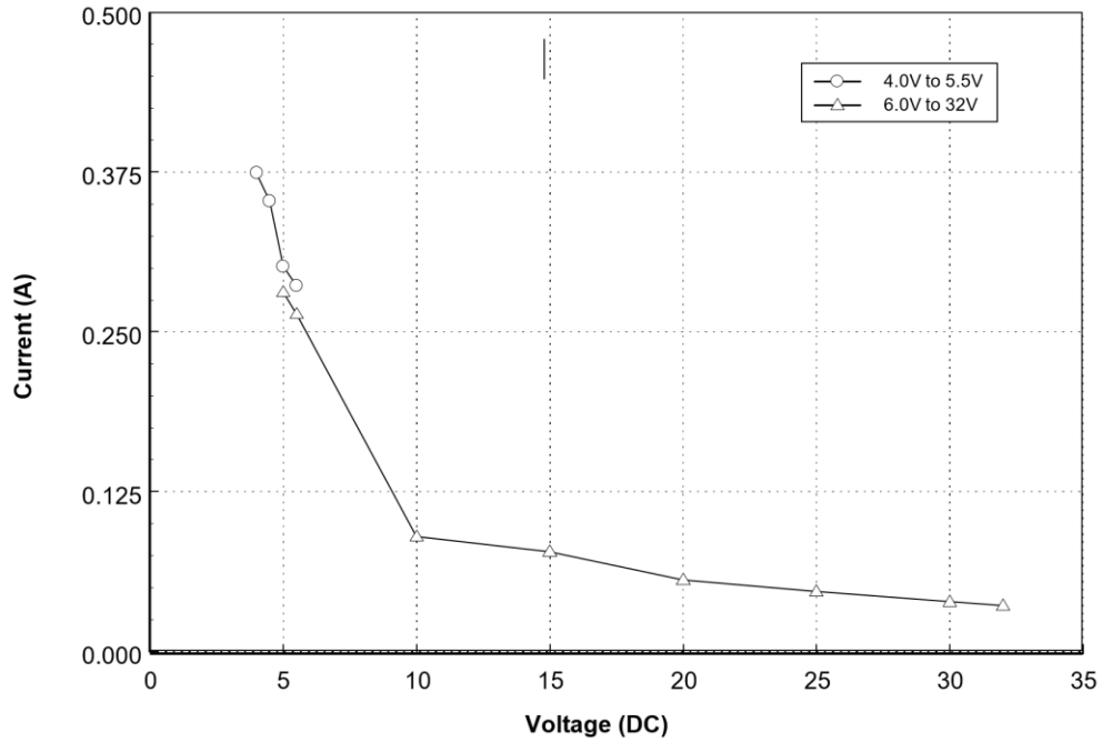
Figure 8: Average Current Drawn During a Data Switch Call
