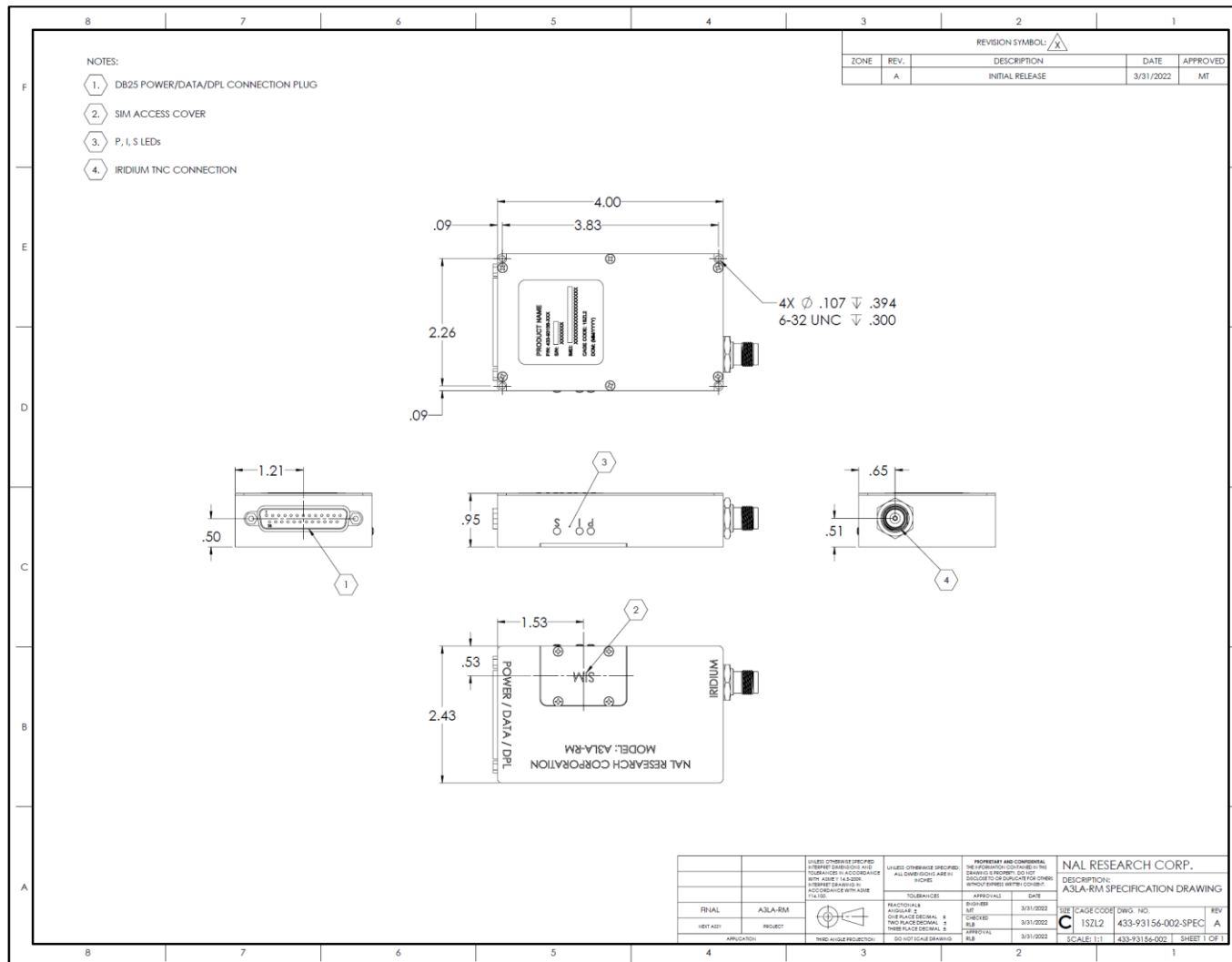
Figure 23: A3LA-RM Mechanical Drawing
