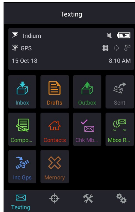
Figure 19: Texting Menu
