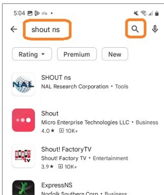
Figure 4: Search Screen
