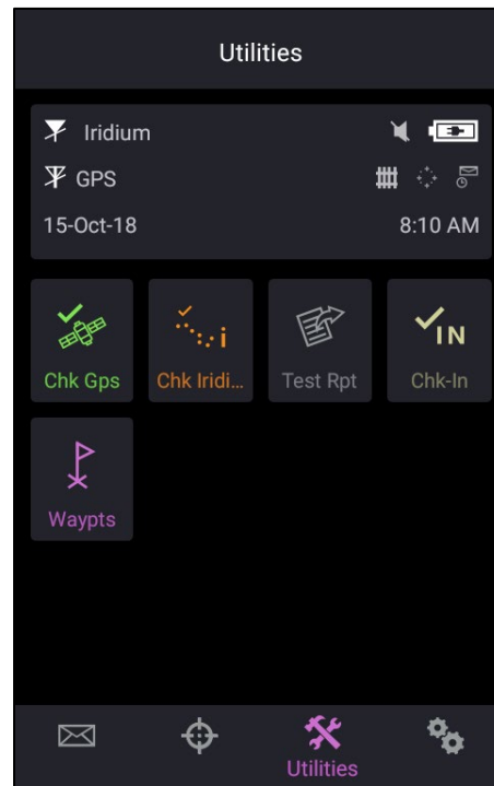
Figure 39: Utilities Menu
