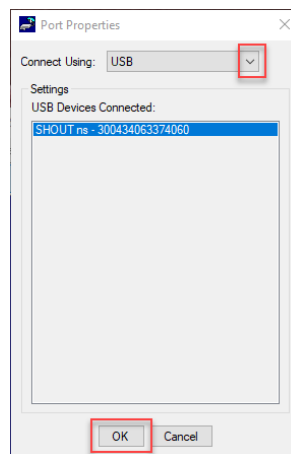
Figure 13: Port Properties
