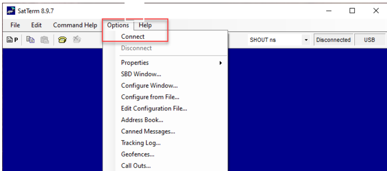
Figure 15: Options>Connect
