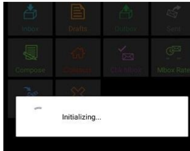
Figure 10: Initializing Device
