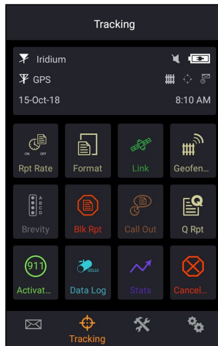
Figure 33: Tracking Menu
