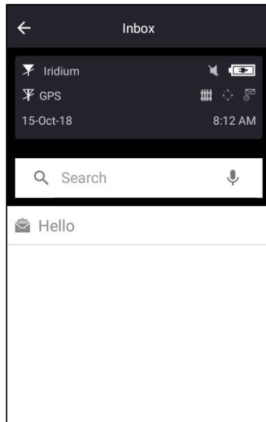
Figure 20: Inbox
