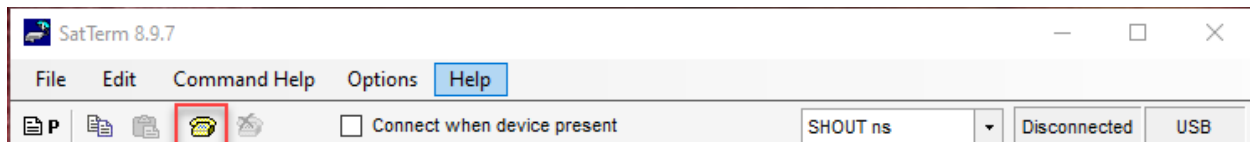
Figure 14: Telephone Icon
