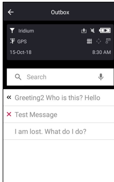
Figure 22: Outbox
