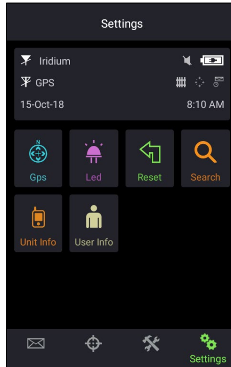
Figure 43: Settings Menu
