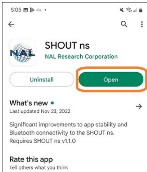
Figure 6: Open Screen
