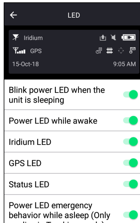
Figure 47: LED Screen
