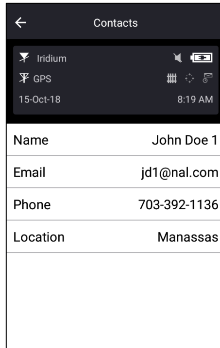
Figure 30: Contact Selected
