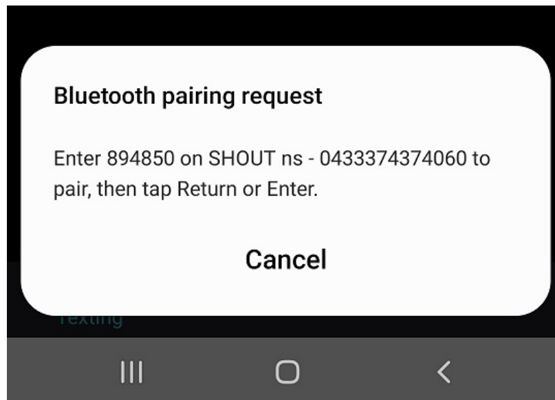
Figure 17: Device Connected
