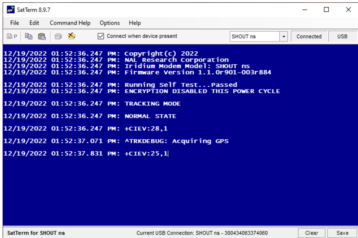
Figure 16: Device Connected
