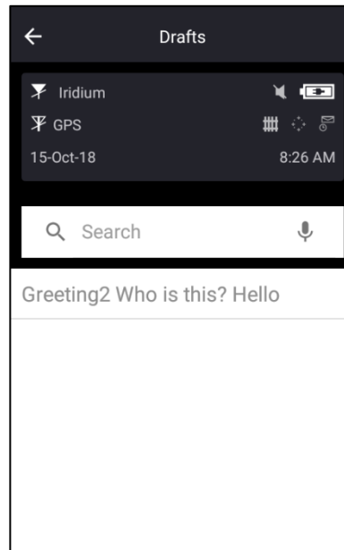
Figure 21: Drafts
