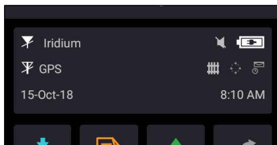
Figure 18: Status Bar
