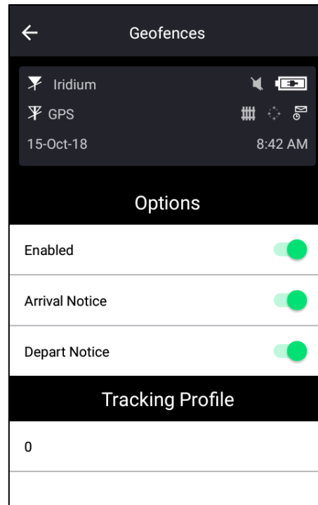
Figure 38: Geofence Options
