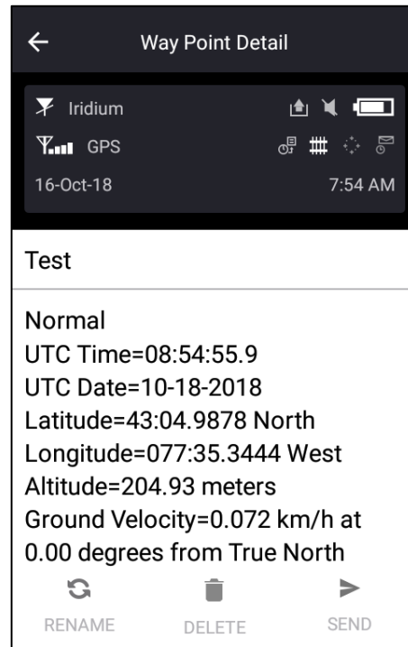
Figure 42: Waypoint Selected
