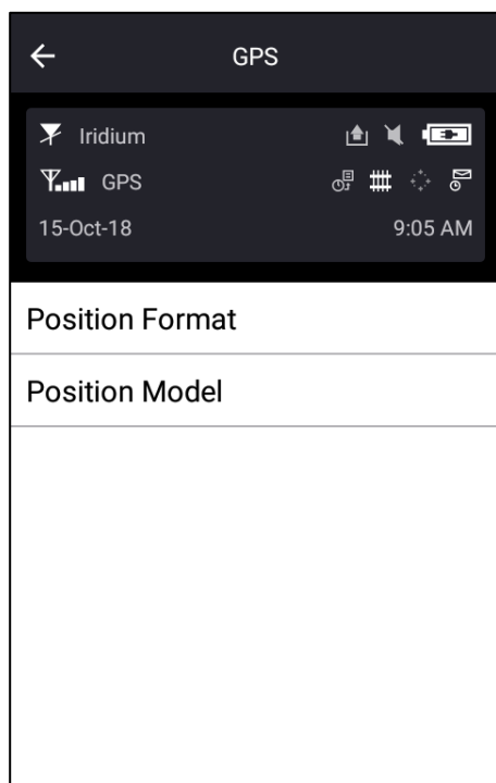
Figure 44: GPS Screen
