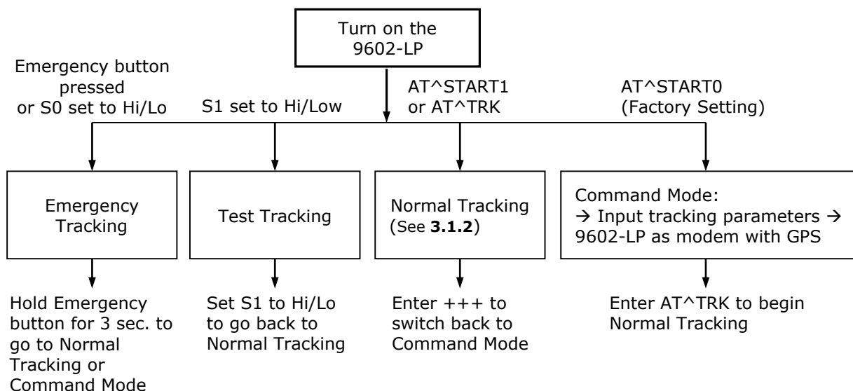
Figure 7: Different Operating Modes of the 9602-LP
