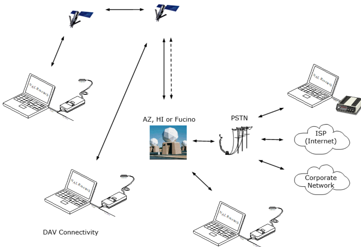
Figure 40: Iridium Dial-Up Data Service
