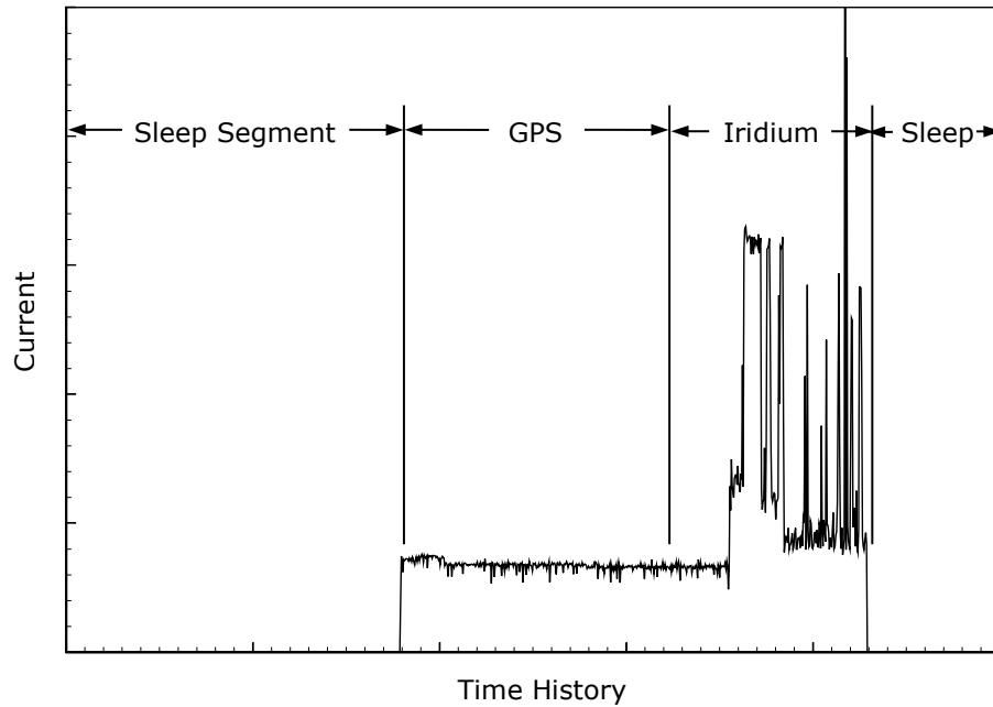
Figure 27: Stages of Current Drawn: Tracking Mode
