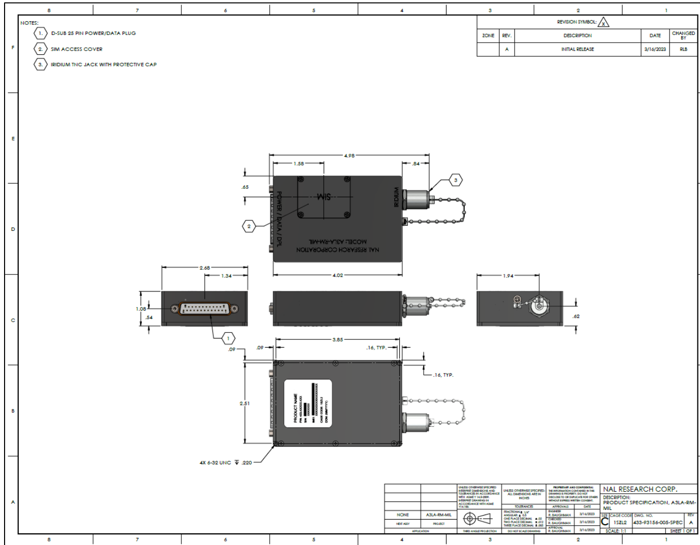
Figure 25: A3LA-RM Mechanical Drawing
