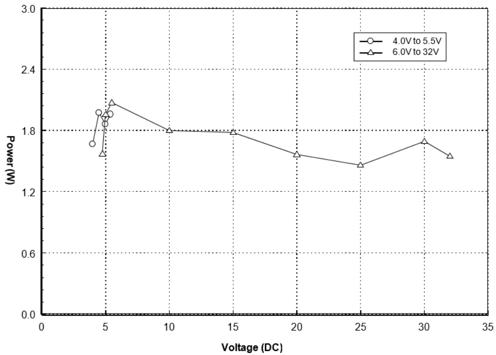
Figure 17: Average Power Consumption During an SMS Transmission
