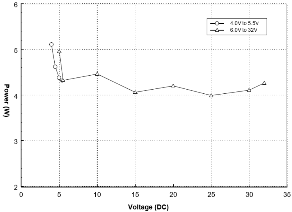
Figure 19: Average Power Consumption During a Voice Call Using DPL Handset
