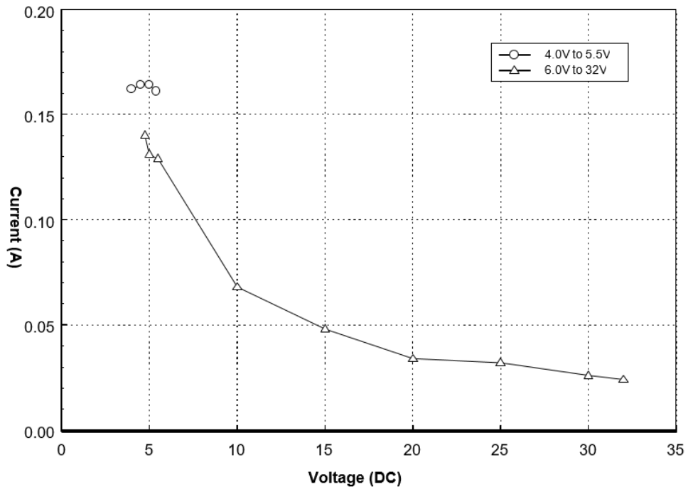
Figure 8: Average Current Drawn During Standby
