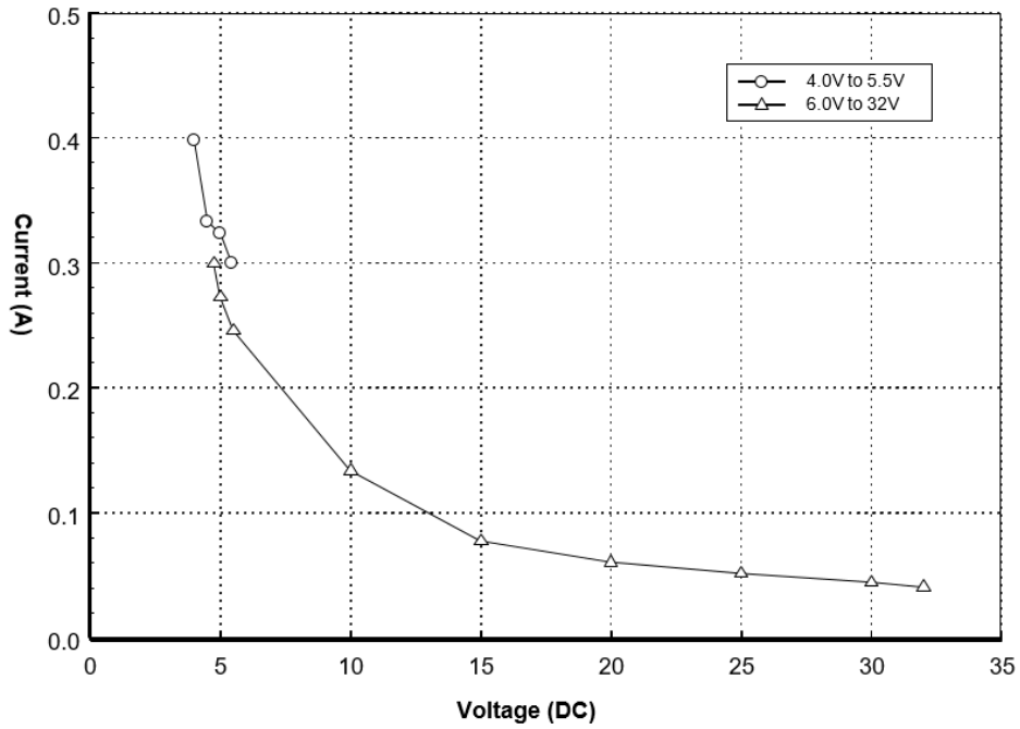
Figure 14: Average Current Drawn During an SBD Transmission
